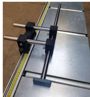
GRADUATED GUIDAL - Axial load < 50 KgF
